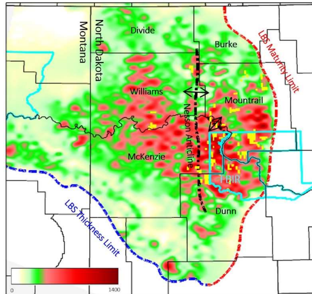
Bakken/Three Forks IP365 (bopd)
